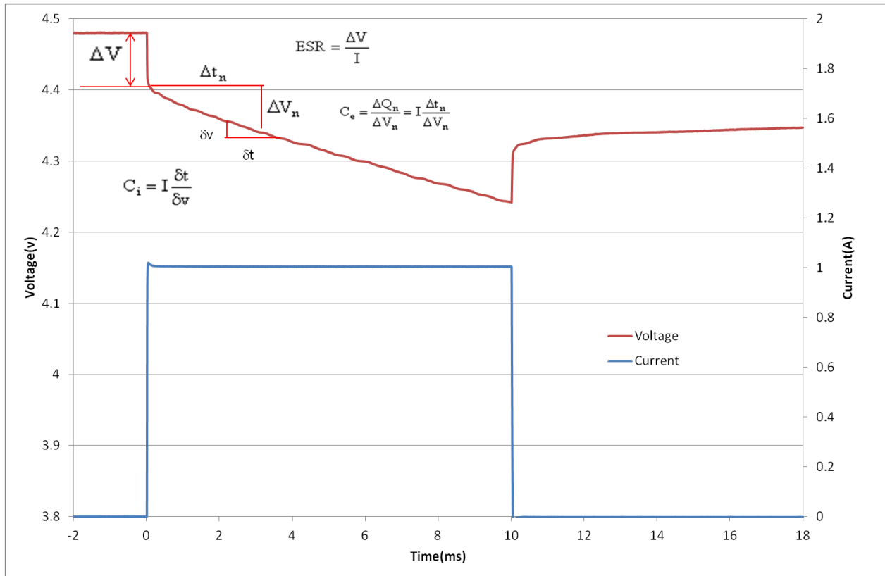
Figure 1: Effective capacitance, instantaneous capacitance and ESR for a GA209
