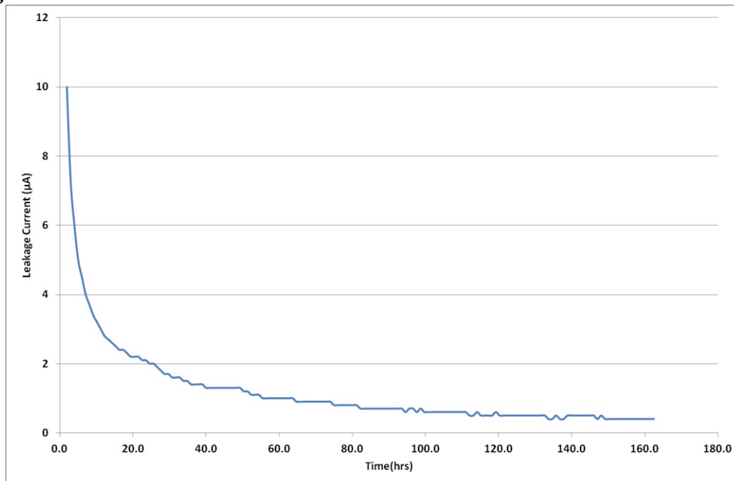
Fig 10: Leakage Current
