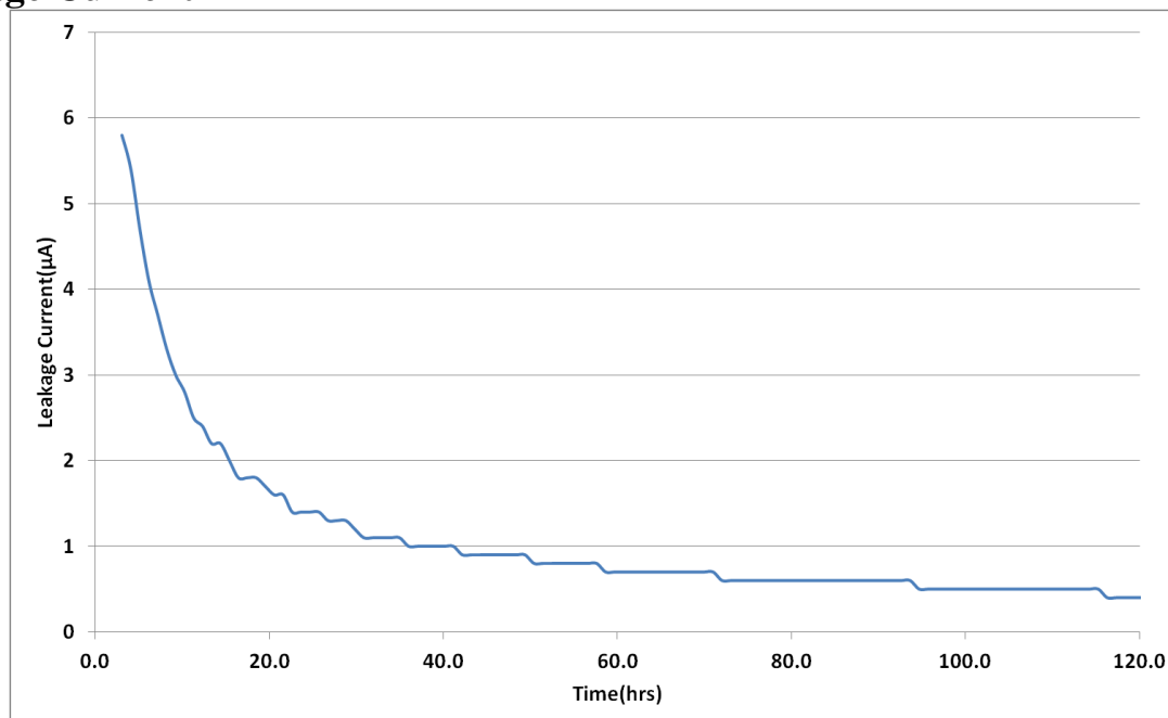
Fig 10: Leakage Current
